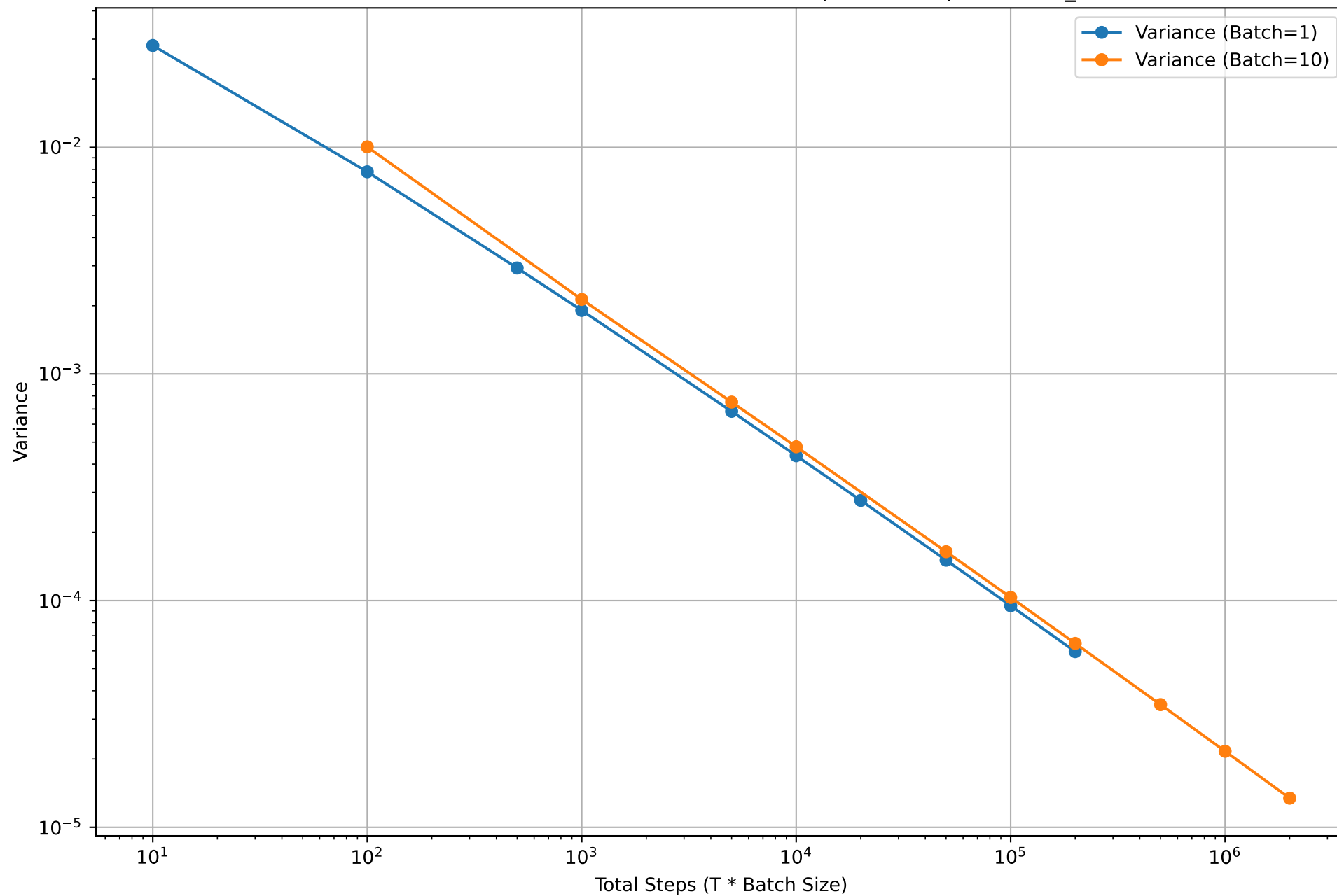
Slock Biases and Variances for Different Batch Sizes; \alpha=1.8 . optiized eta_star for each T
